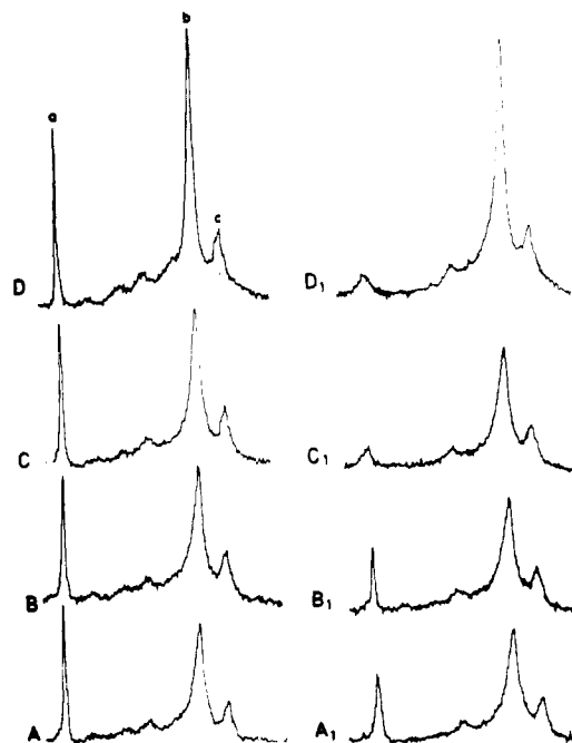
FIGURE 8: ^1\text{H} NMR spectra of sonicated dispersions of 20 mM PC with various concentrations of DOC (A, 0; B, 6; C, 12; D, 16 mM). Spectra A 1 –D 1 were recorded following the addition of \text{MnCl}_2 to a concentration of 0.1 mM. For peak assignment see Figure 3.
