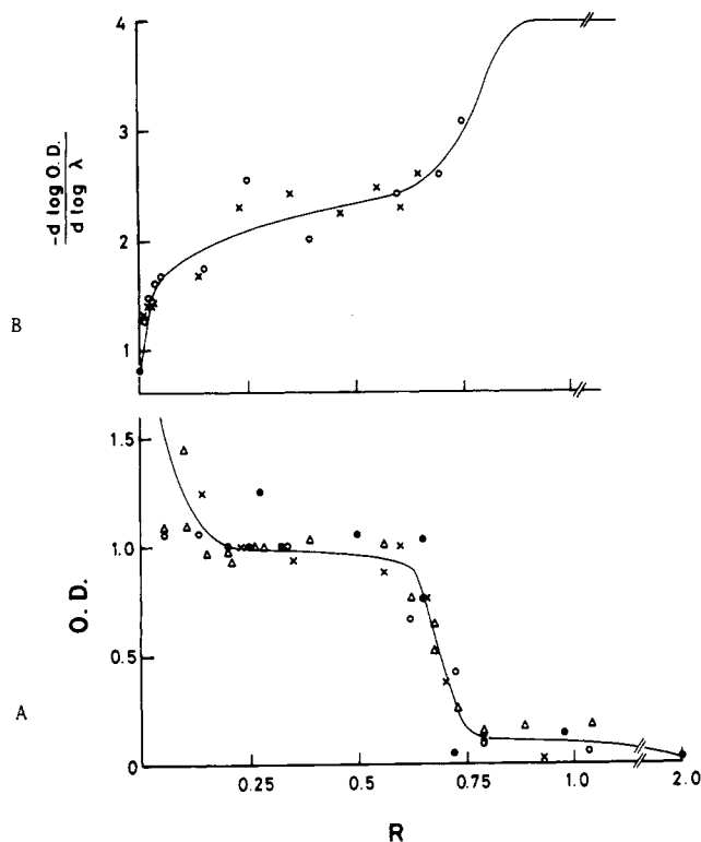
FIGURE 9: The dependence of turbidity parameters (A, OD; B, -\frac{d \log OD}{d \log \lambda} ) on the molar ratio of DOC to PC ( R ) for various PC concentrations. (●) 20; (×) 10; (○) 5; (△) 1 mM.
