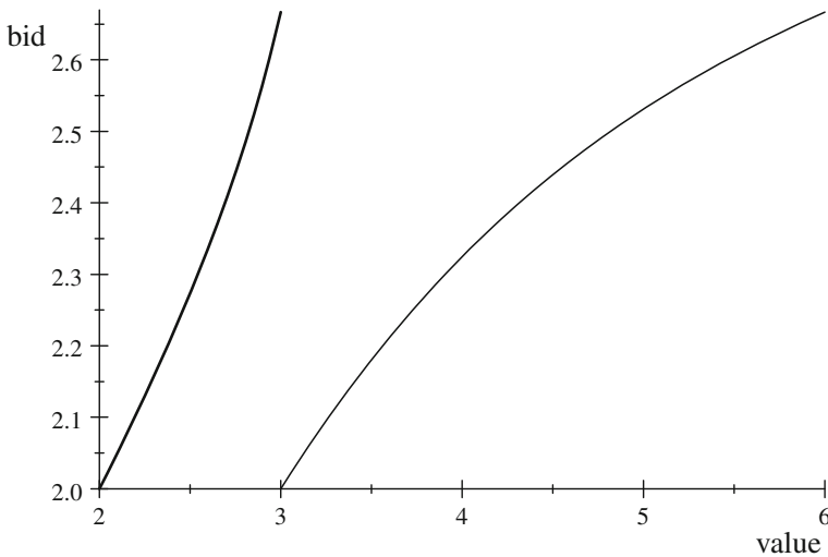
Fig. 4 Solution to Example 4, \underline{v}_1 = 0 , \underline{v}_2 = 3 , m = 2 , \bar{v}_1 = 3 , \bar{v}_2 = 6 . The thicker line is v_1(b)
