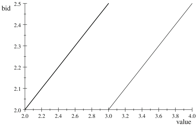
Fig. 3 Solution to Example 3 when \underline{v}_1 = 0 , \underline{v}_2 = 3 , m = 2 , \bar{v}_1 = 3 , \bar{v}_2 = 4 . The thicker line is v_1(b)
