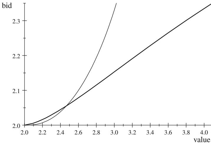
Fig. 1 Solution to Example 1, \underline{v}_1 = 0 , \underline{v}_2 = 1 , m = 2 , \bar{v}_2 = 3 , \bar{v}_1 = 4 . The thick line is v_1(b)
