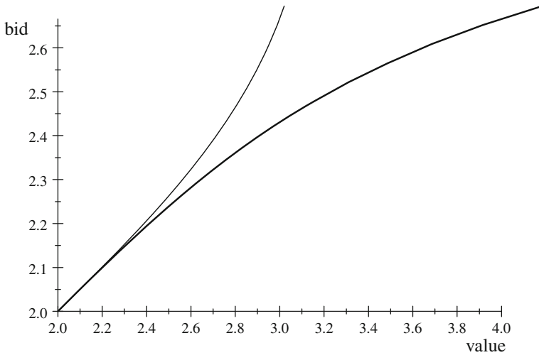
Fig. 2 Solution to modified Example 1 when \underline{v}_1 = 2 , \underline{v}_2 = 2 , \bar{v}_2 = 3 , \bar{v}_1 = 4 . The thicker line is v_1(b)
