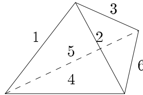
Figure 2: Tetrahedral net
