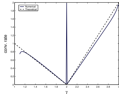
FIG. 4: Convergence rate.
