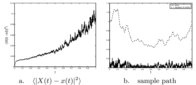
FIG. 3: Difference between the solution of the limiting equation and the equation of motion for \gamma = 3 , for \epsilon = 0.1 .
