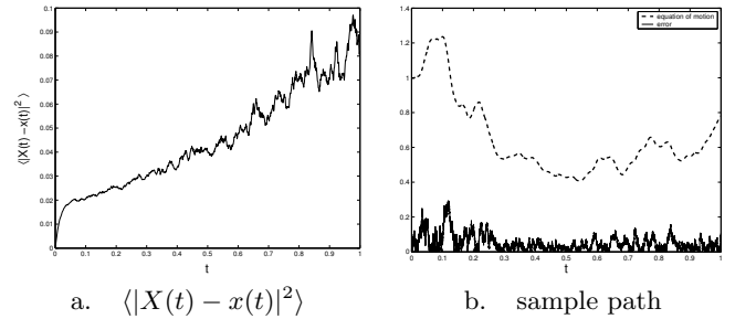
FIG. 2: Difference between the solution of the limiting equation and the equation of motion for \gamma = 2 , for \epsilon = 0.1 .
