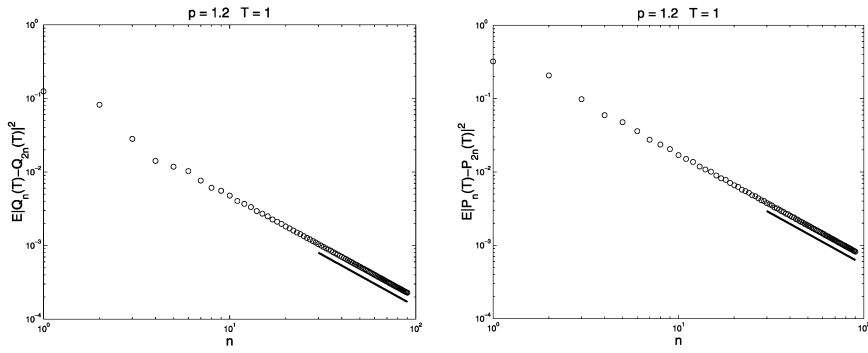
Fig. 1. Log-log plot of the mean square deviations, E |Q_{2n}(t) - Q_n(t)|^2 (left) and E |P_{2n}(t) - P_n(t)|^2 (right), versus n for p = 1.2 and t = 1 . The solid lines have the expected slope of decay of 2p - 1 .
