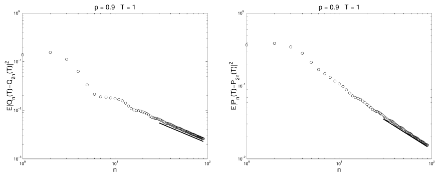
Fig. 2. Same at Fig. 1 for p = 0.9 .
