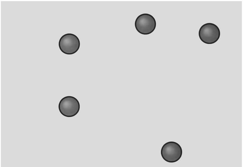
FIG. 1. A society in which all the partitions into two groups are unstable.
